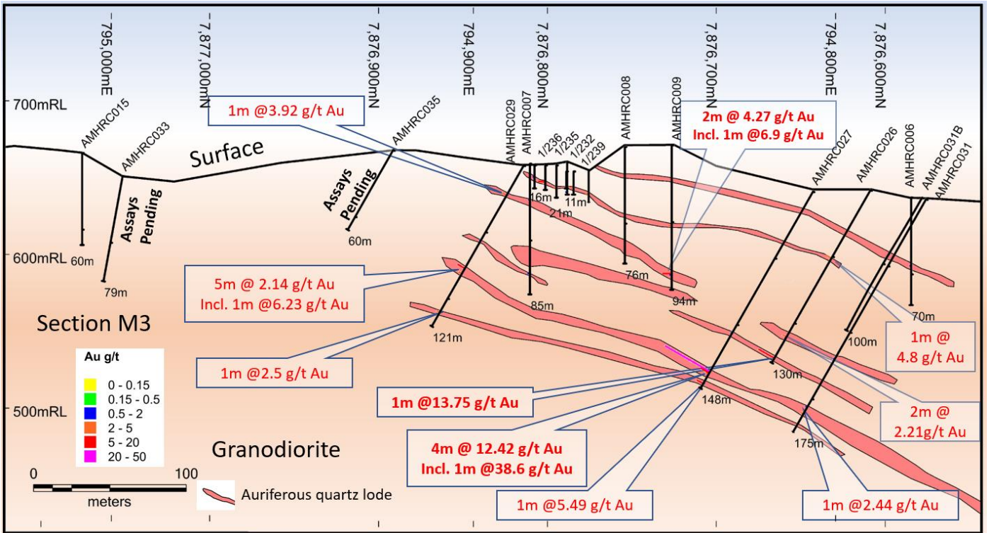
Figure 6. Mt Hogan Historic Gold Mine M3 section
